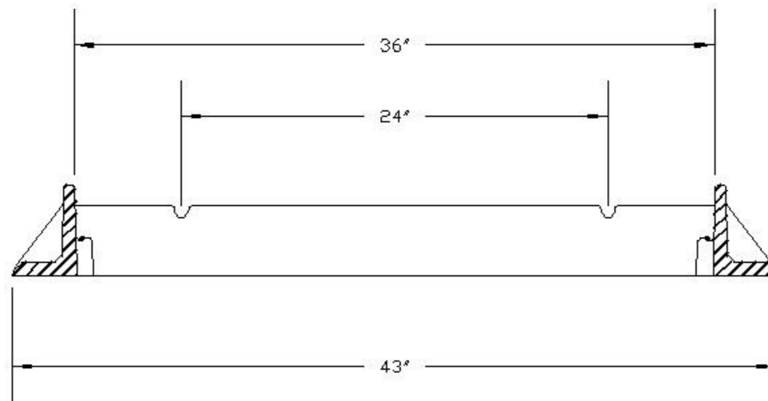
FRAME SECTION
