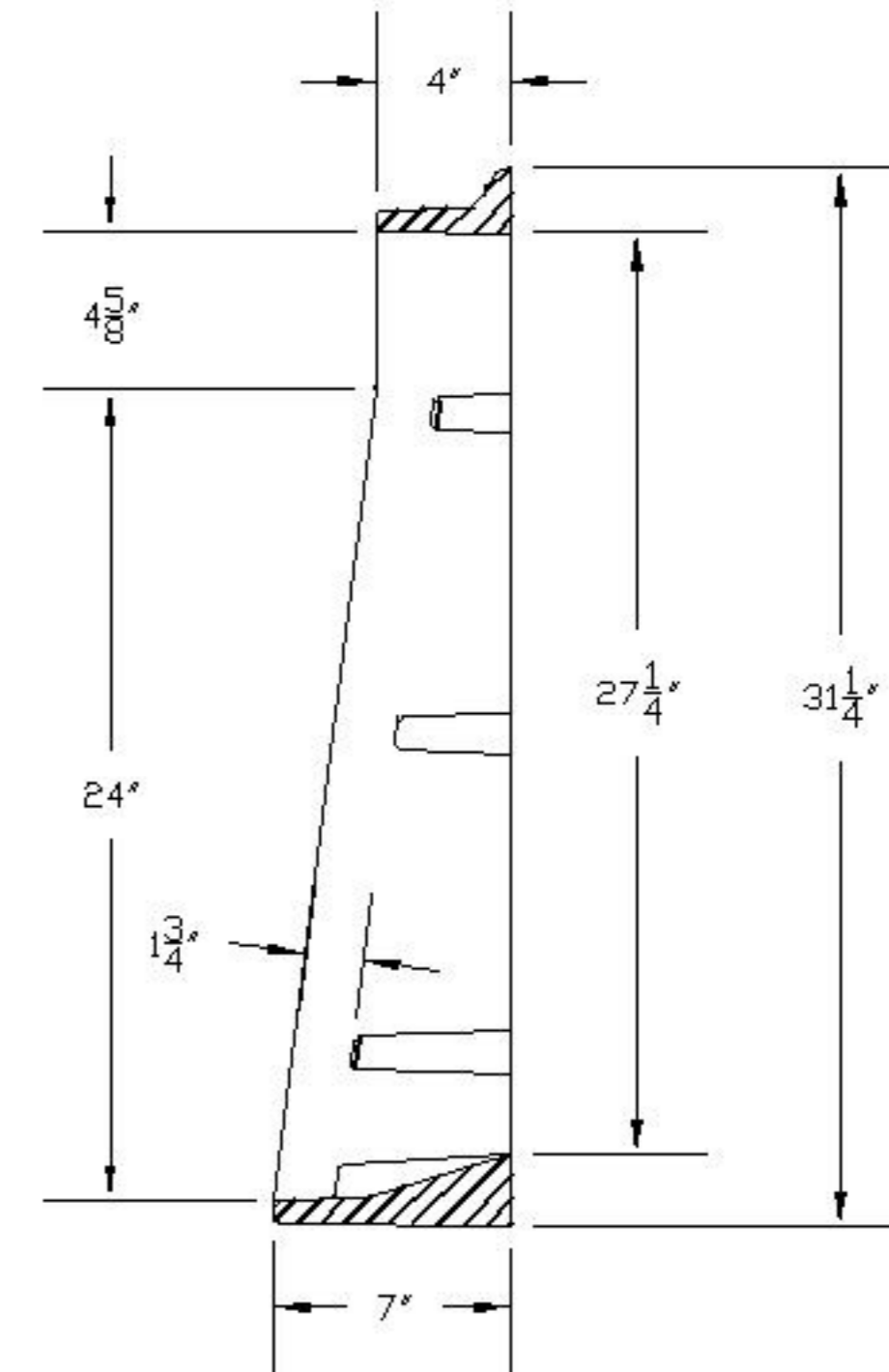
FRAME SECTION
