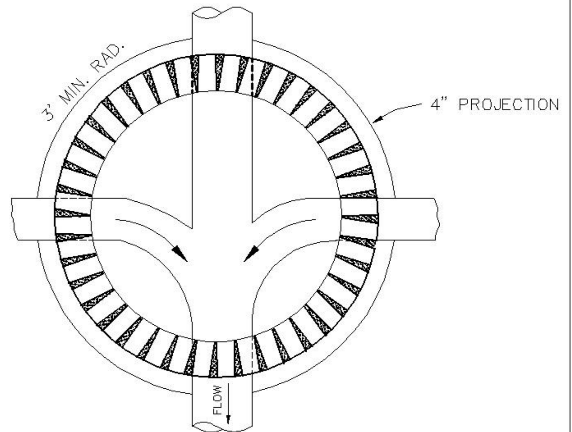
PLAN SHOWING LATERALS SIDE OF CHANNEL TO BE SLOPED 1"/FT
